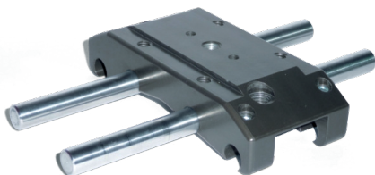
Roll fixture, low profile (FIX 2-0363)
